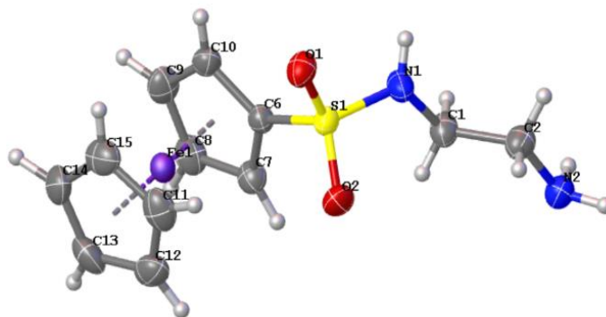
Figure 1. ORTEP of the molecular structure of the compound [(\eta^5-C_5H_5)Fe(\eta^5-C_5H_4SO_2NH-CH_2-CH_2-NH_2)] . Bond distances (Å) selected: C_5H_4 (centroid)-Fe 1.651(4); Fe- C_5H_5 (centroid) 1.656(4); S(1)-N(1) 1.597(3); S(1)-O(1) 1.438(2); S(1)-O(2) 1.436(2); S(1)-C(6) 1.757(3); N(1)-C(1) 1.468(6); N(2)-C(2) 1.468(5); C(2)-C(1) 1.507(5). Angles ( ^\circ ) selected: N(1)-S(1)-O(1) 106.8(1); N(1)-S(1)-O(2) 108.2(1); N(1)-S(1)-C(6) 108.6(2); O(1)-S(1)-O(2) 119.5(1); O(1)-S(1)-C(6) 106.8(1); O(2)-S(1)-C(6) 106.5(1); S(1)-N(1)-C(1) 120.4(3).
