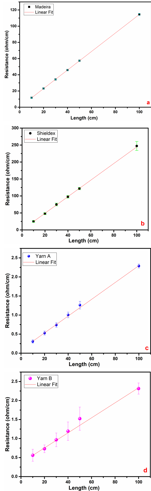
FIGURE 3. Linear Electrical Resistance values of the yarns a) Madeira, b) Shieldex, c) Yarn A, and d) Yarn B.
