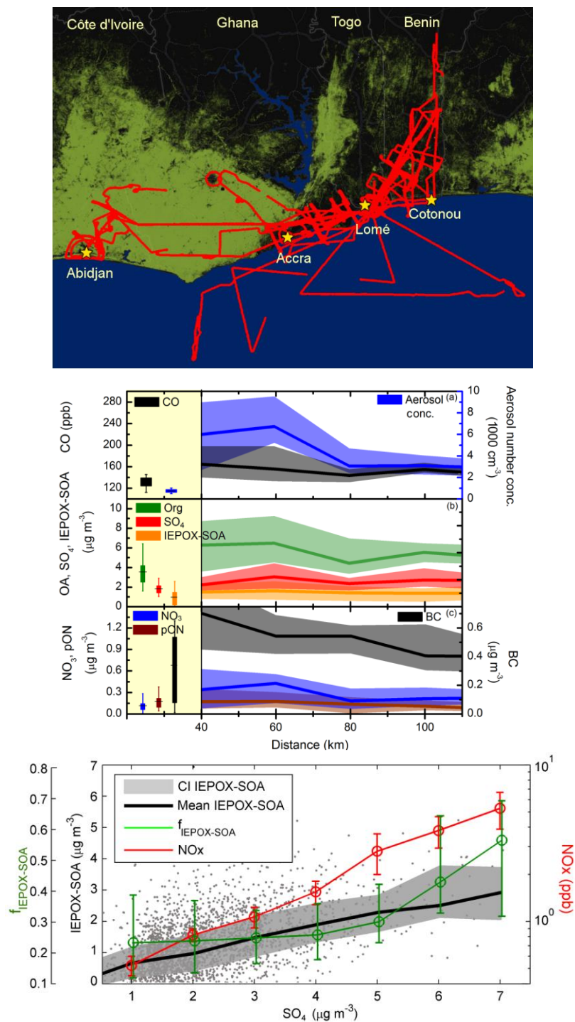
Figure 3.3.3 – Top: ATR42 trajectories (in red) during DACCIWA for altitudes below 2000 m overlaid the forest cover (in green), non-forested areas (black) and water surface (blue). Middle: Regional background (marked in yellow) and in-plume concentrations for CO and aerosol concentration (a); OA, SO 4 and IEPOX-SOA (b); and NO 3 , pON, and BC (c). Bottom: Scatterplot between IEPOX-SOA concentration and SO 4 . The black line and grey area represent the mean and 5 and 95 % confidence intervals of the mean, respectively. Red and green markers are mean NO x and f IEPOX-SOA , respectively. Reproduced from Brito et al. (2018).
