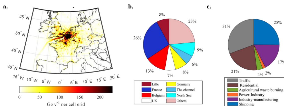
Figure 3.1.10 – a) Accumulated contribution of BC to ATOLL in Gg\ y^{-1} per cell grid and its regional (b) and sectorial (c) distribution over the period Dec 2016 – Dec 2019.
