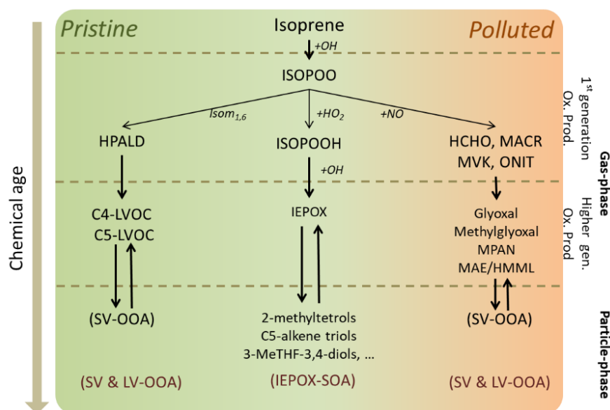
Figure 3.3.1 – Schematic diagram of isoprene photooxidation. In the presence of \text{NO} , isoprene oxidation favours the \text{NO} route. At low \text{NO} levels, \text{ISOPOO} can be scavenged along the \text{HO}_2 pathway, or undergo isomerization when \text{NO} and \text{HO}_2 concentrations are sufficiently low. The \text{HO}_2 route can lead to isoprene epoxydiols ( \text{IEPOX} ), an efficient aerosol-forming compound.
