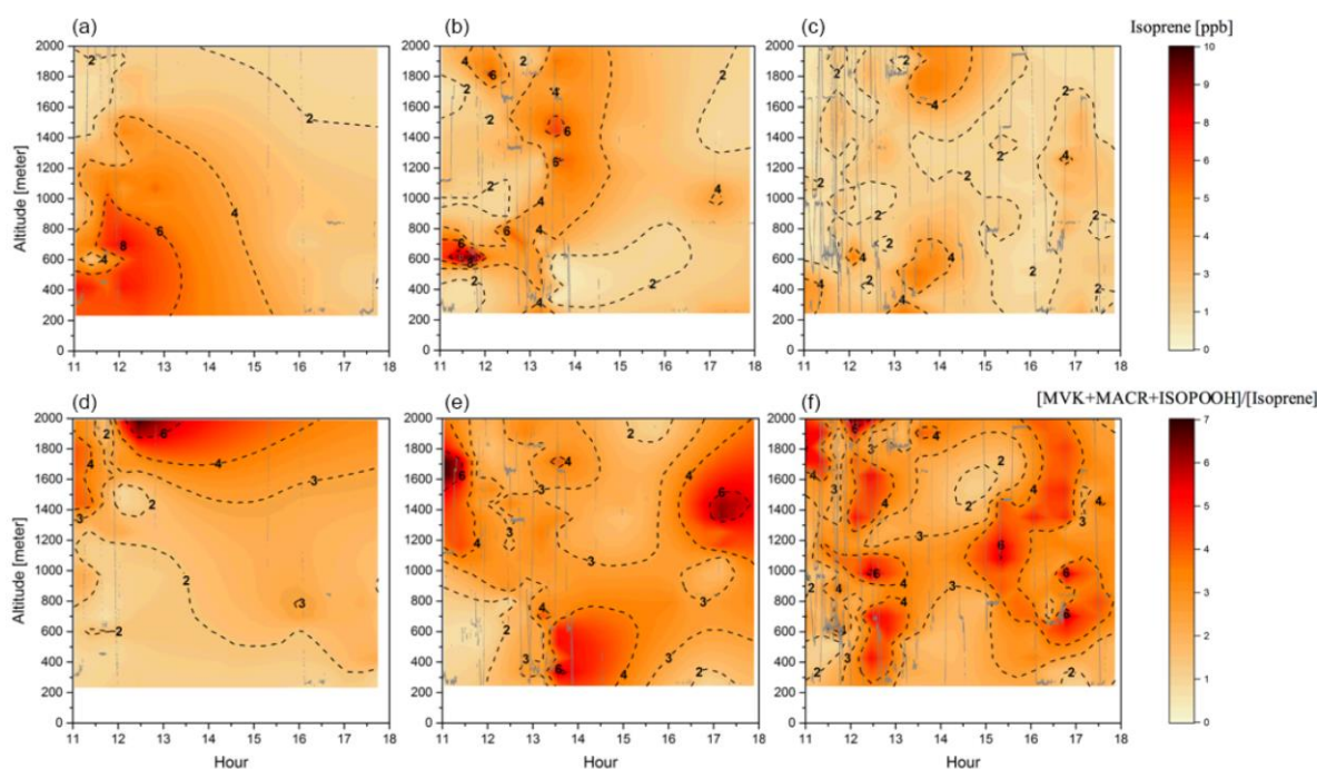
Figure 3.2.5 – Cross section of the isoprene mixing ratio (ppbv) (a–c) and the [MVK+MACR+ISOPOOH] / [isoprene] ratio (d–f) for the three different groups: background environment (on the left), fresh smoke plume ( t < 2 h, middle), and aged smoke plume ( t > 2 h, on the right). Hour is in local time. Reproduced from Santos et al. (2018).
