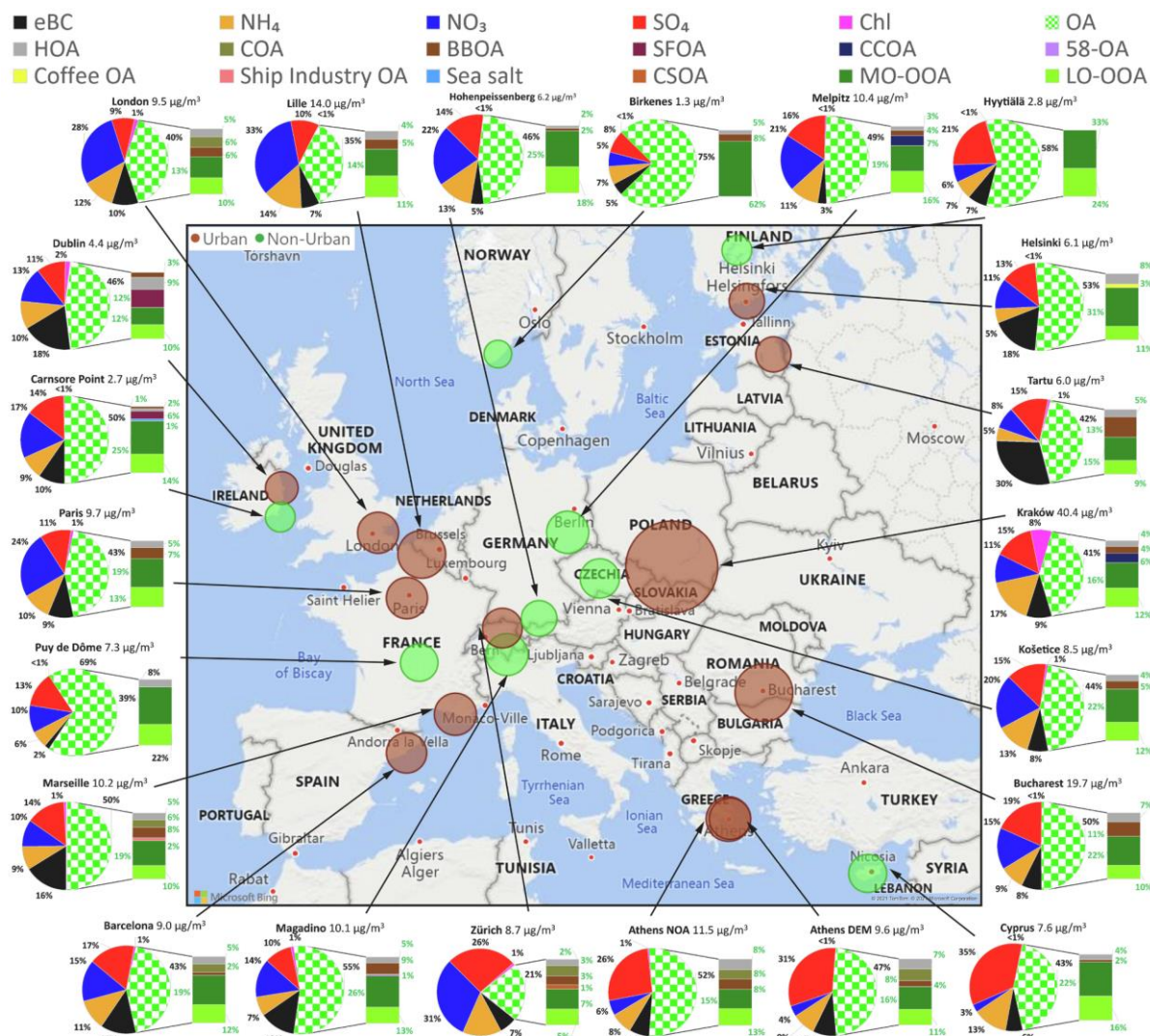
Figure 3.1.12 – PM 1 mass fractions of non-refractory inorganic species, BC and OA covering all seasons. The size of the markers corresponds to the PM 1 mass concentration. The brown colour of the marker indicates an urban site, while the green marker indicates a non-urban site. The checkered green/white shading of the pie charts denotes the OA fraction in PM 1 , and the bar charts represent the contributions of each OA factor to the total OA mass. COA stands for cooking-like OA, CCOA for coal combustion OA, SFOA for solid fuel OA (mainly mixture of coal and peat combustion), 58-OA a specific source associated with Amines, and CSOA for cigarette smoke OA. ATOLL is identified here as "Lille". Reproduced from (Chen et al., 2022).
